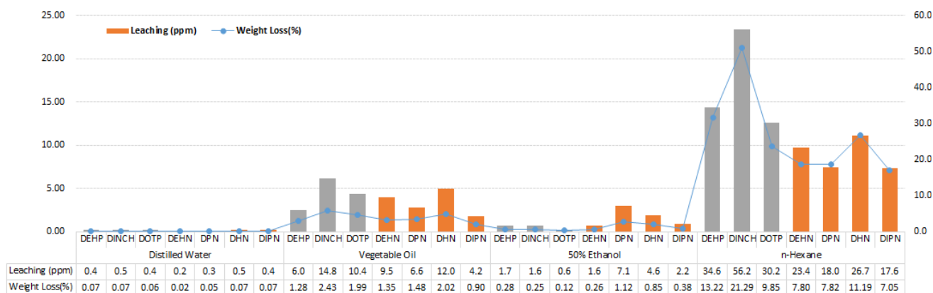
Figure 1. Migration test results of PVC films containing synthesized compounds into various solvents.
